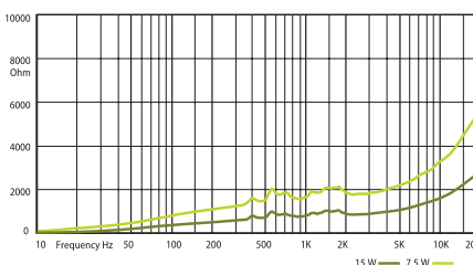
IMPEDANCE
